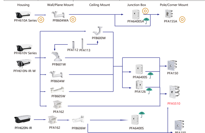
Camera Housing Wall/Plane Mount Ceiling Mount Junction Box Pole/Corner Mount
