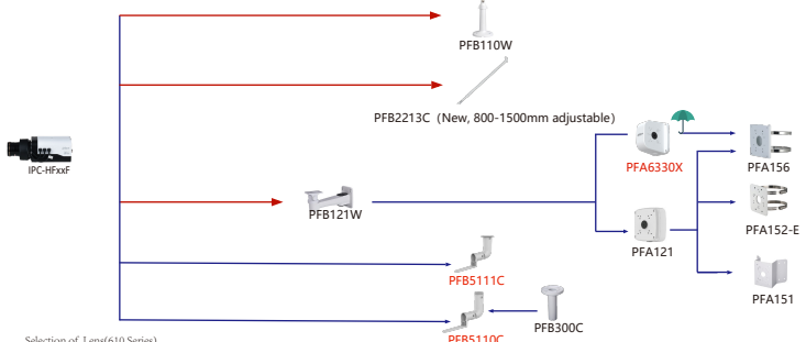
Selection of Lens(Box Camera)
