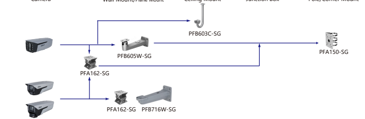
Camera Wall Mount/Plane Mount Ceiling Mount Junction Box Pole/Corner Mount
